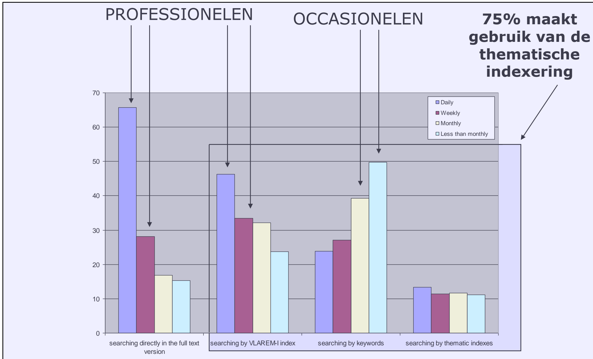
Fig. 2 Relation searching method and user frequency
